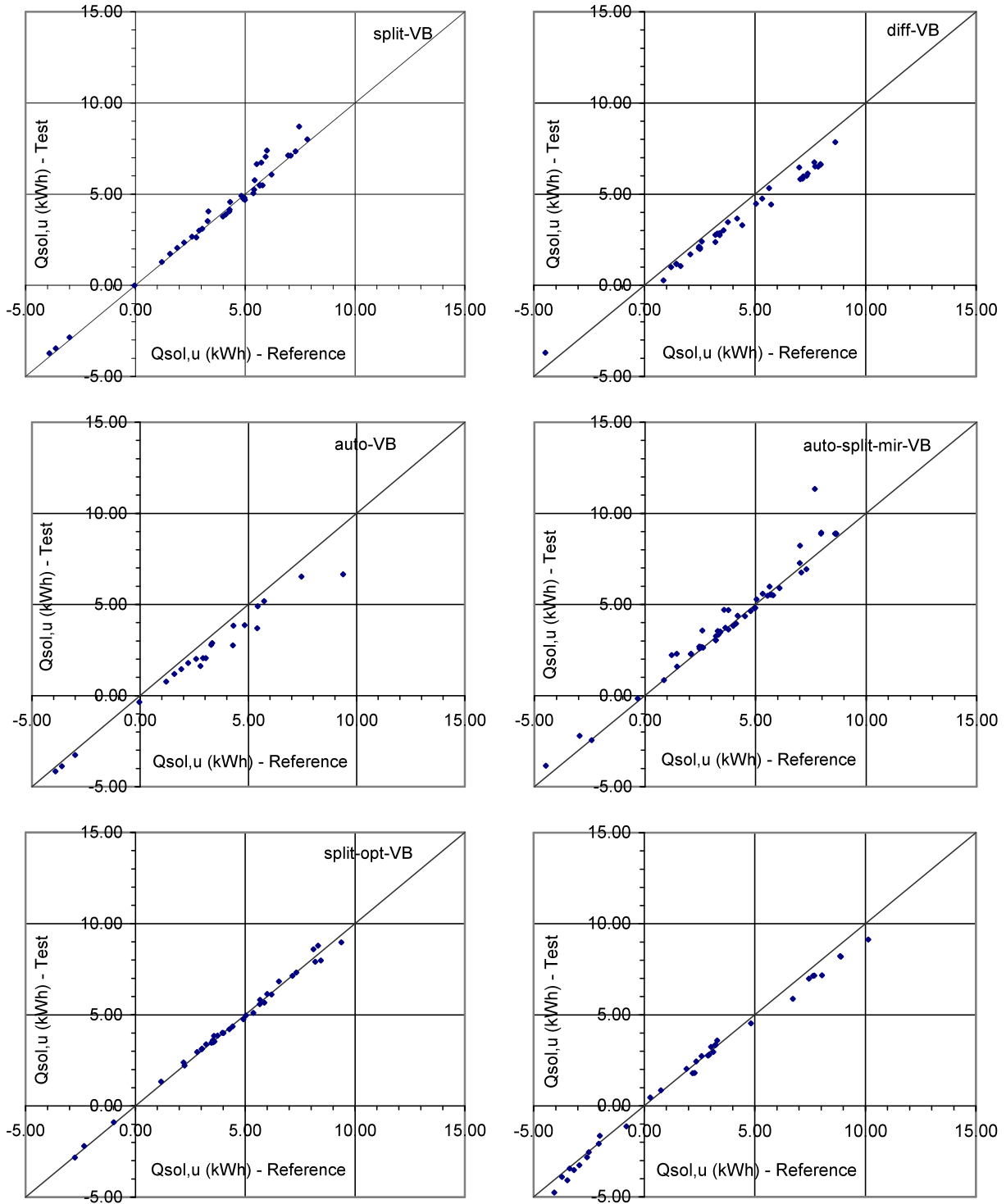
Figure 12: Interior shading: Daily cooling load due to solar and thermal heat gains through the window (kWh) over the 6:00-18:00 period.
