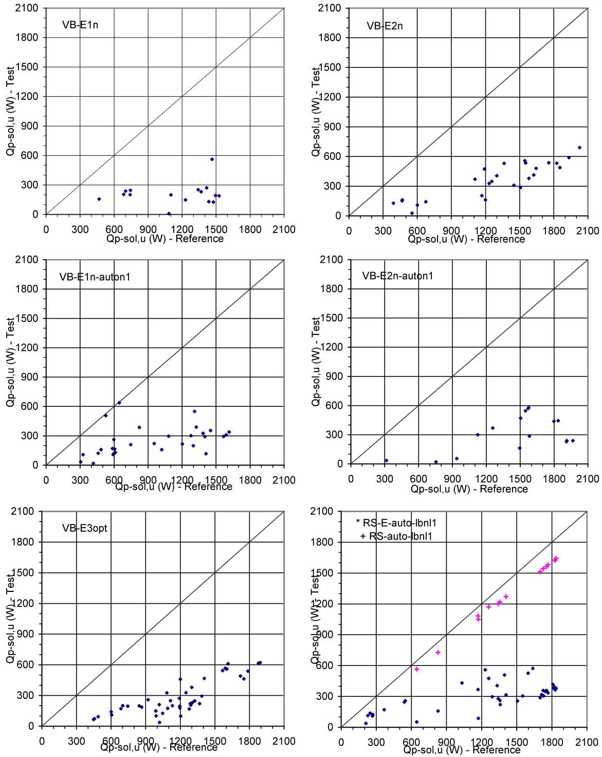
Figure 22: Exterior shading: Peak cooling load due to solar and thermal heat gains through the window (W).
