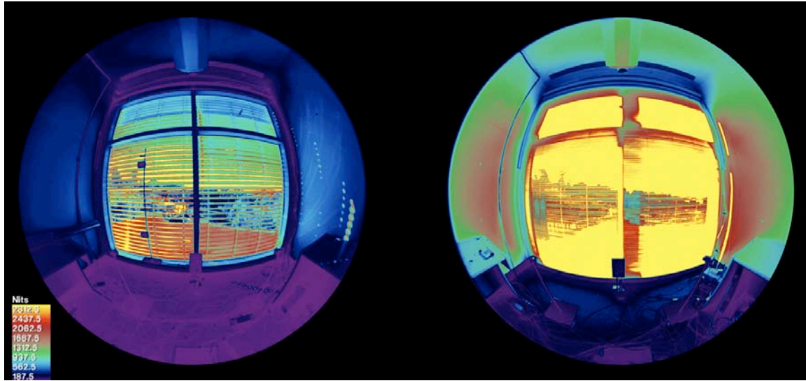
Figure 24: Left: (VB-E3opt), right: reference interior Venetian blind (ref-VB). March 22, 10:02 solar time, “clear” sky conditions. Falsecolor luminance threshold (yellow) \geq 3000 cd/m 2 .
