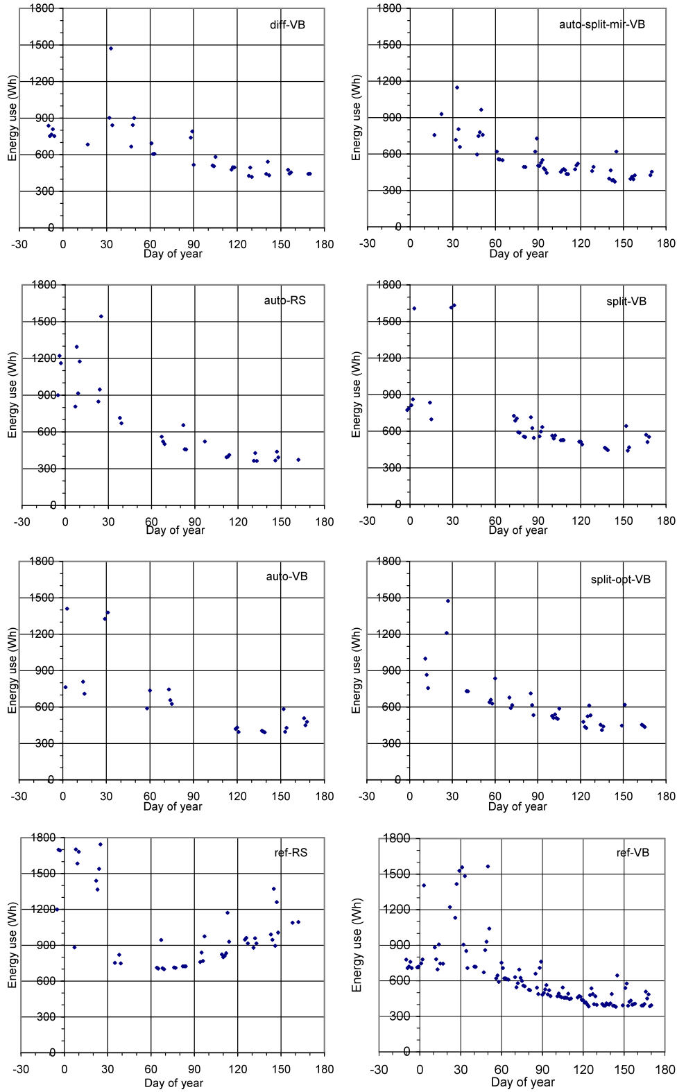
Figure 11: Interior shading: Daily lighting energy use (Wh) per test condition for the 6:00-18:00 period.
