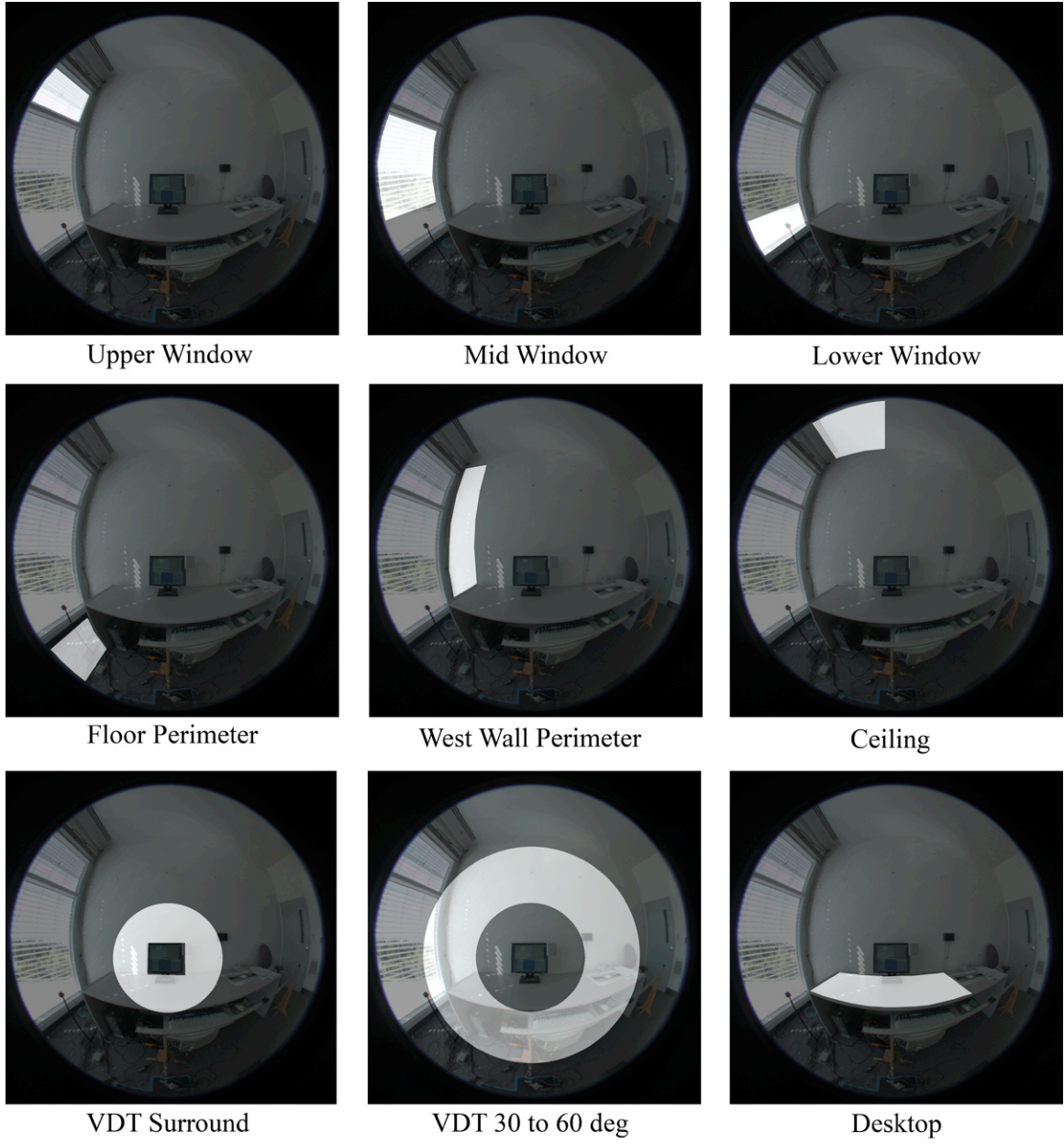
Figure 10: The average luminance for each of the above zones was computed from each HDR image using a bitmap mask (VDT-view).
