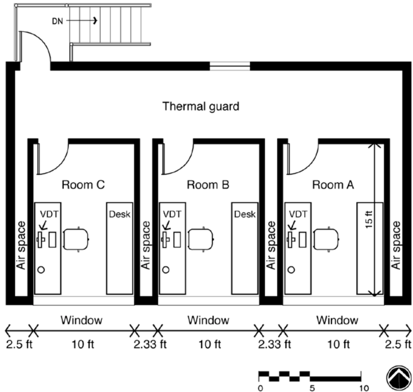
Figure 7: Floor plan of the LBNL Windows Testbed Facility
