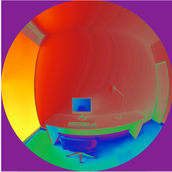
a) Falsecolour luminance map ( \text{cd}/\text{m}^2 ) rendered with the use of BSDF data. Matte-VB: January 15, 10:00 AM.
