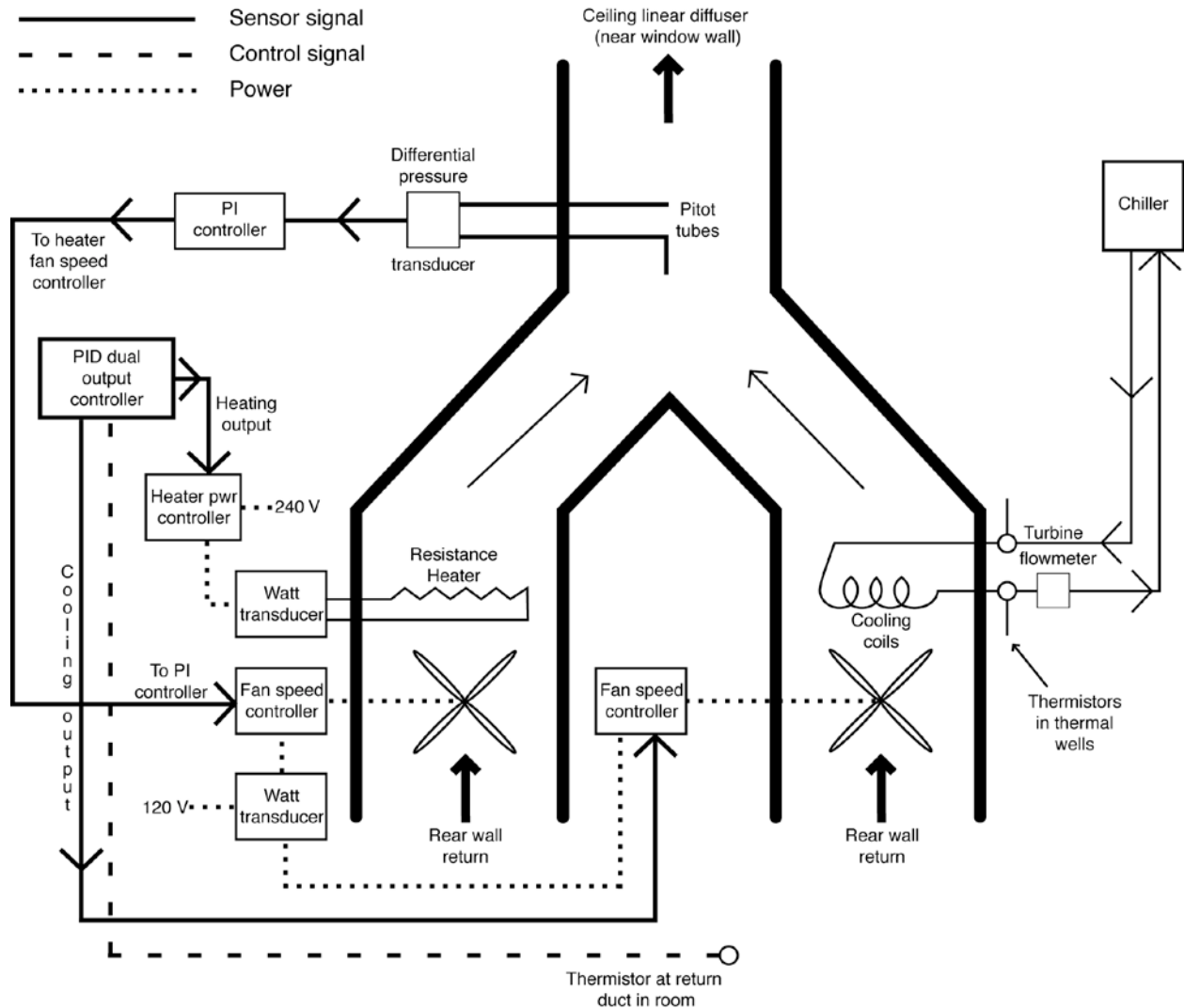
Figure 8: Schematic of HVAC system in the LBNL Windows Testbed Facility
