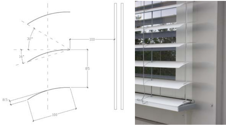
Figure 4: Vertical cross-section view of exterior Venetian blind (VB-E1n). Dimensions are given in millimeters.
