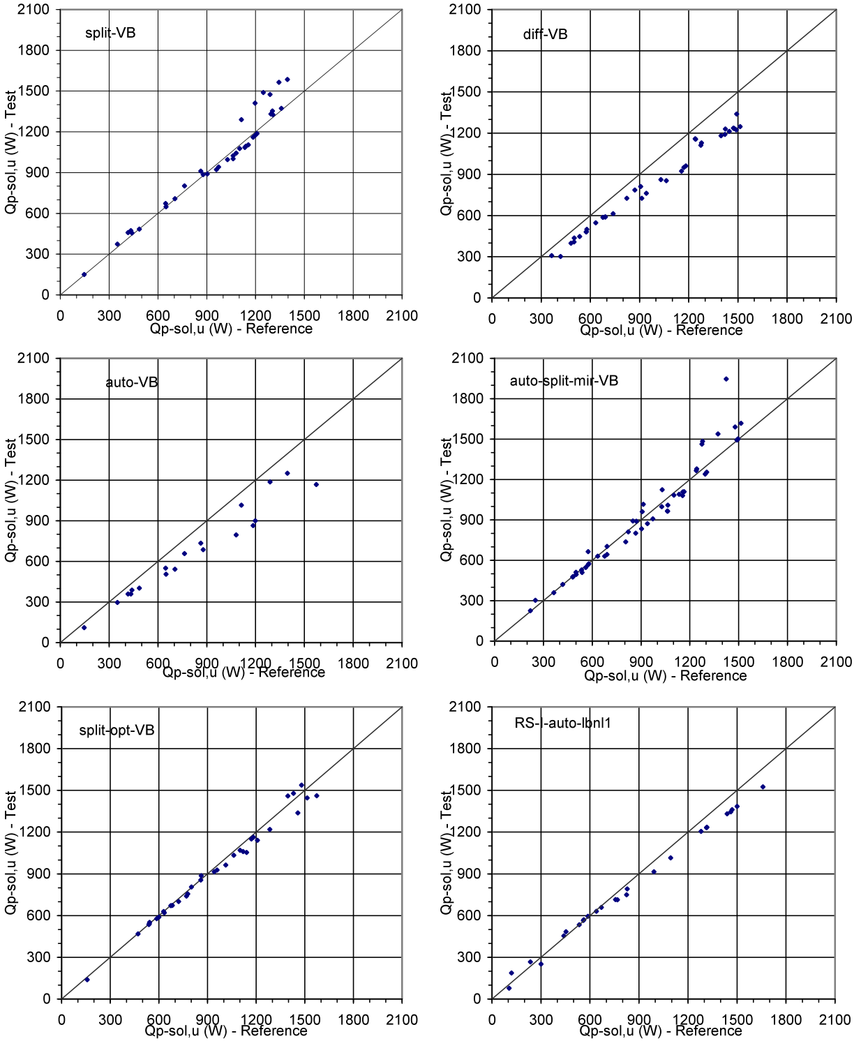
Figure 13: Interior shading: Peak cooling load due to solar and thermal heat gains through the window (W).
