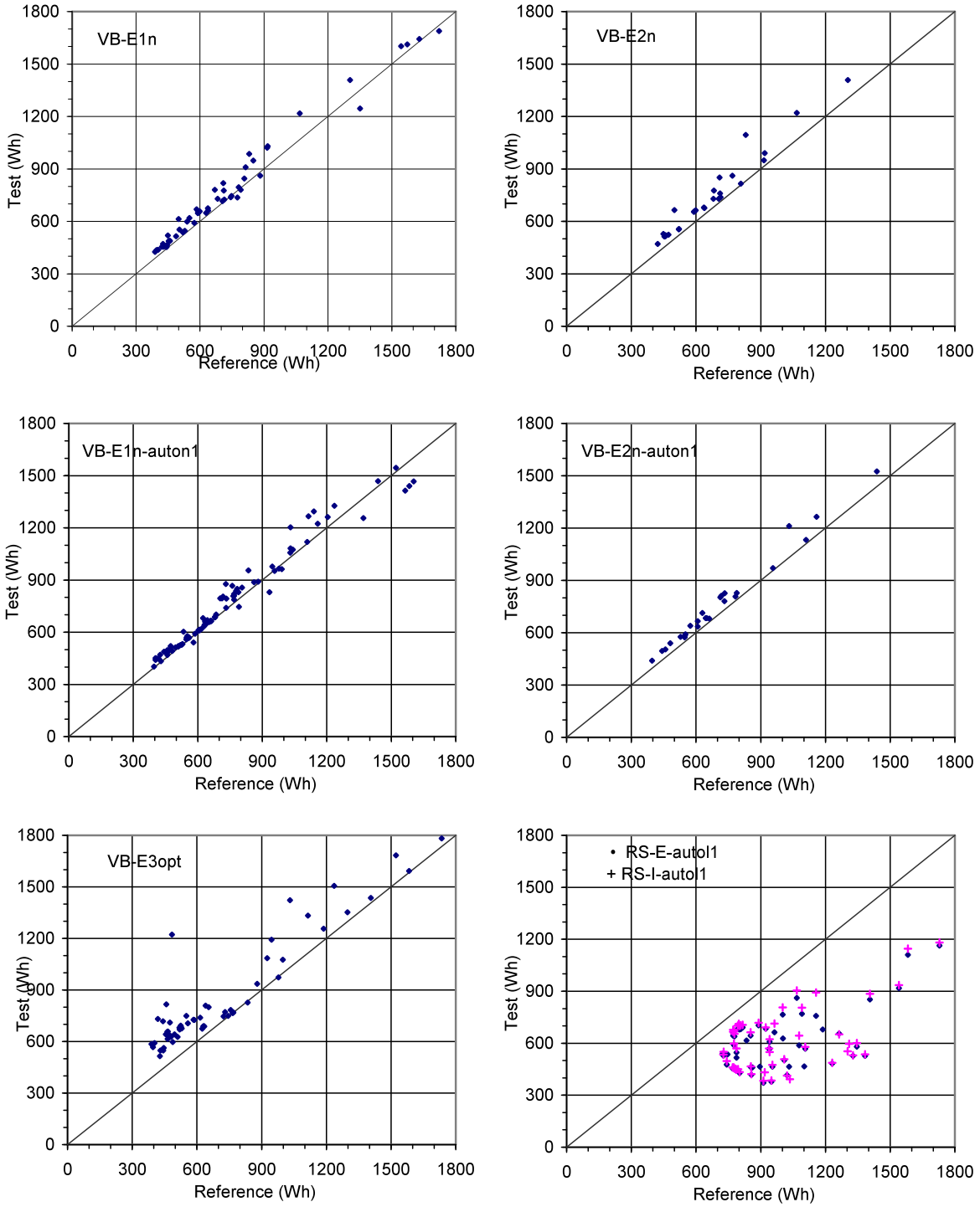
Figure 20: Exterior shading: Daily lighting energy use (Wh) per test condition for the 6:00-18:00 period.
