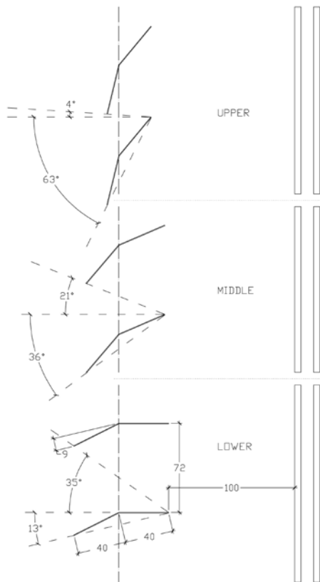
Figure 5: Vertical cross-section view of exterior Venetian blind (VB-E3opt). Dimensions are given in millimeters.
