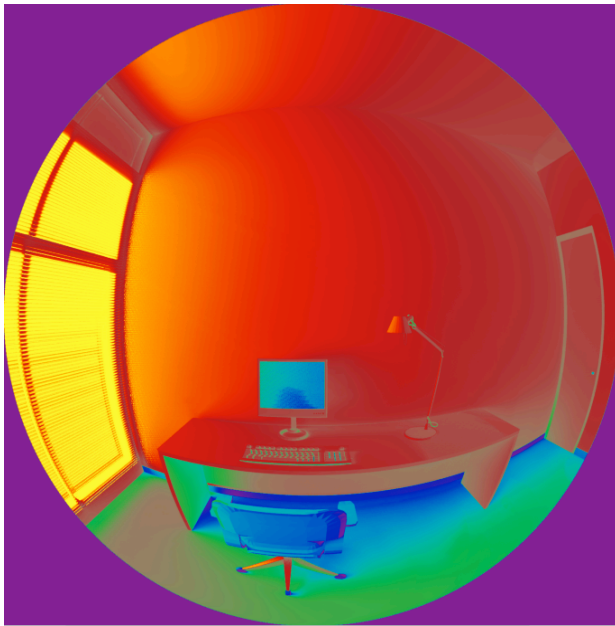
b) Falsecolour luminance map ( \text{cd}/\text{m}^2 ) rendered without use of BSDF data. Matte-VB: January 15, 10:00 AM.
