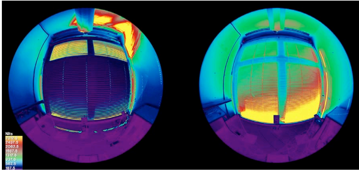
Figure 16: Left: Automated split optical Venetian blind (auto-split-mir-VB). Right: reference Venetian blind (reference-VB). February 4, 10:02 AM. Falsecolor luminance threshold (yellow) \geq 3000 \text{ cd/m}^2 .
