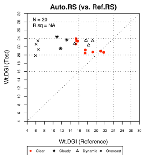
Figure 19: Interior shading: Visual comfort performance (window view) for test condition (y-axis) versus reference condition (x-axis) for all sky conditions.
