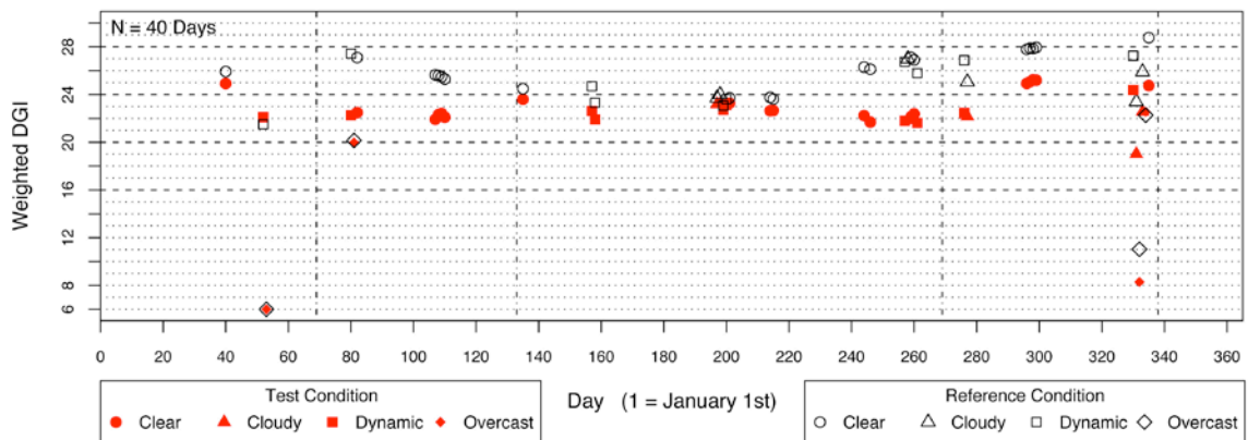
Figure 26: Weighted DGI values of paired comparisons for all sky conditions over the two 6-month test periods. Vertical lines indicate the dates of seasonal adjustment of blocking angle for the ref-VB only. The blocking angle for each section of the VB-E3opt was fixed in the same position for both test periods.
